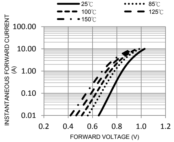
FIG. 2-Typical Forward Characteristics
